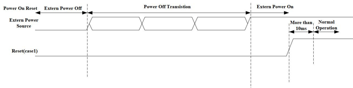
H/W reset pin timing for power-on reset
